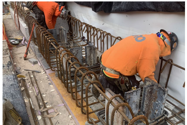
Capbeam installation at 600 W. 125th Street
